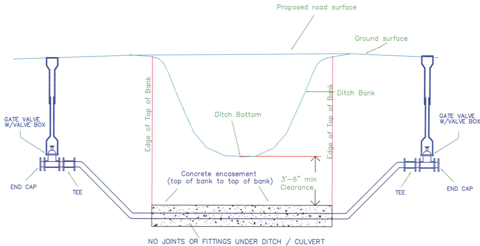
A-A TYPICAL DRAWING FOR REROUTING W.M. @ CULVERT / DITCH
