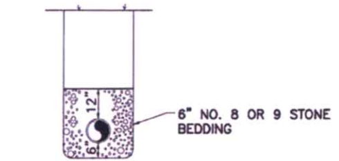
TRENCH DETAIL
